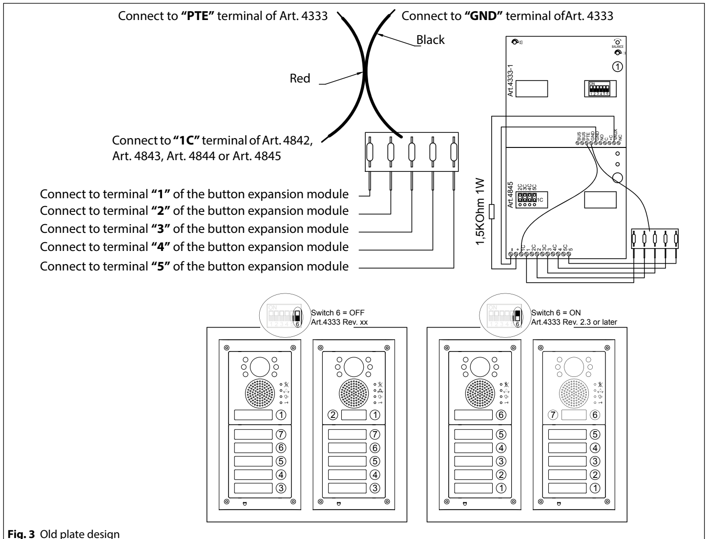
Fig. 3 Old plate design
