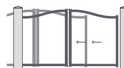
2-leaf imitation for sliding gate
